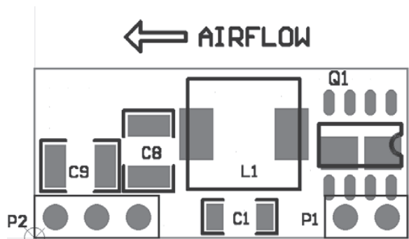
Figure 7. Temperature Measurement Location for SIP
